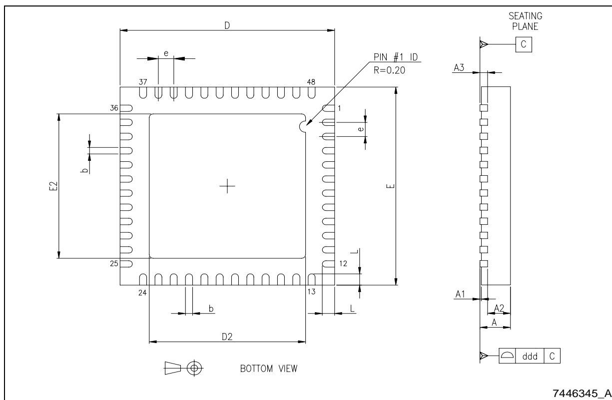
VFQFPN-48 (7x7x1.0mm) Very Fine Quad Flat Package No lead
